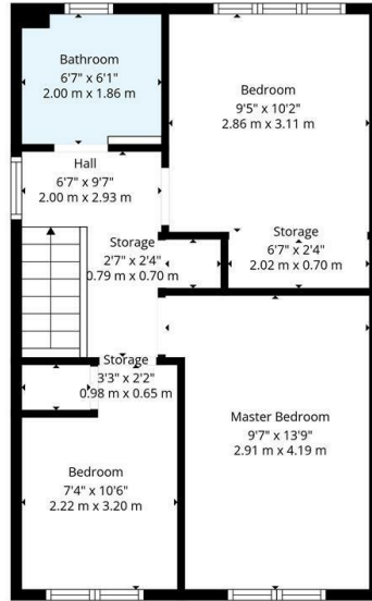
2nd Floor
